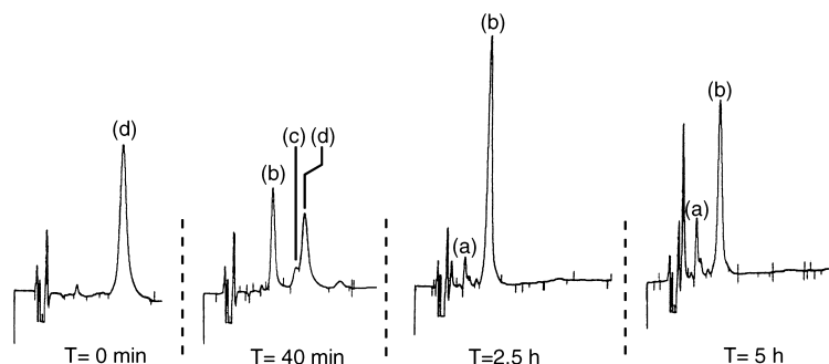
Figure 1. Separation of T-IP 5 ( 2 ) and the phosphatidylinositol intermediates, T-IP 4 , T-IP 3 , and T-IP 1 , produced during the 3-phytase catalyzed dephosphorylation of T-IP 5 , was achieved by reversed phase ion pair chromatography. Where (a) = T-IP 1 ( t_R 3.9 min); (b) = T-IP 3 ( t_R 5.8 min); (c) = T-IP 4 ( t_R 7.7 min), and (d) = T-IP 5 ( 2 ) ( t_R 8.5 min).
