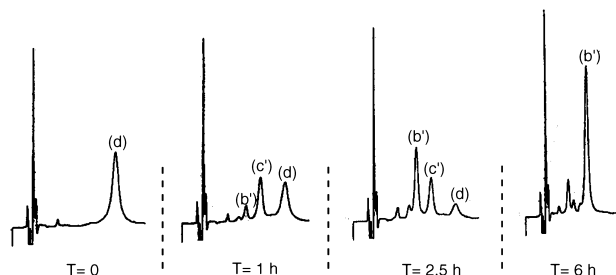
Figure 4. Separation of tethered (T)-IP 5 ( 2 ) and the phosphatidylinositol intermediates produced during the 6-phytase catalyzed dephosphorylation of T-IP 5 was achieved by reversed phase ion pair chromatography. Where (b') = T-IP 3 ( t R 6.9 min); (c') = T-IP 4 ( t R 8.6 min), and (d) = T-IP 5 ( 2 ) ( t R 11.2 min). Note that primes are used, since T-IP 3 and T-IP 4 may be different isomeric forms of the compounds referred to in Figure 1. The ratio of the MeOH–H 2 O component of the mobile phase was 57:43.
