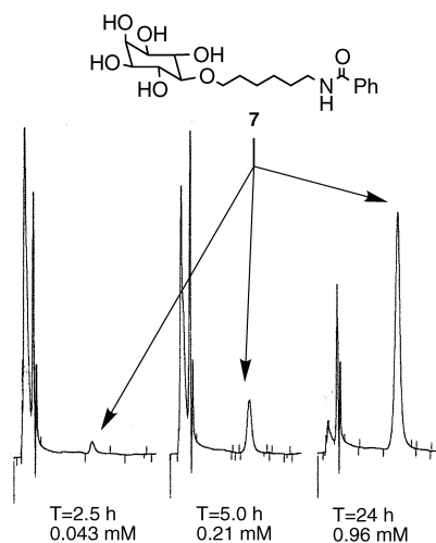
Figure 3. HPLC chromatograms illustrating the appearance of T- myo -inositol (7) from the 3-phytase dephosphorylation assay of T-IP 5 (2). T- myo -inositol was separated on a PRP-1 reversed phase column using MeOH–H 2 O. The concentration of the T- myo -inositol (7) was determined by use of an authentic standard.
