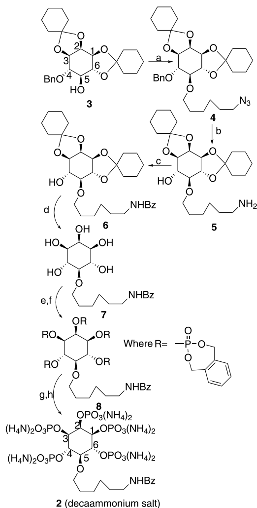
Scheme 1. Synthesis of T-IP 5 ( 2 ). Reagents and conditions: (a) MsO(CH 2 ) 6 N 3 (2.5 equiv), NaH (2 equiv), DMF, 55 °C, 16 h (97%); (b) 10% Pd/C, THF–MeOH (1:1), H 2 , 50 psi, 8 h (55%); (c) BzCN (1.1 equiv), CH 2 Cl 2 , 16 h, rt (76.6%); (d) HOAc, H 2 O, 100 °C, 24 h (94%); (e) N,N -diethyl-1,5-dihydro-2,4,3-benzodioxaphosphepin-3-amine (7 equiv), tetrazole (10.5 equiv), MeCN, 24 h; (f) 11 equiv MCPBA, –50 to 25 °C (88%, two steps); (g) 5% Pd/C, MeOH, THF, H 2 O, H 2 , 50 psi; (h) 10 equiv NH 3 (95.8%, two steps).
