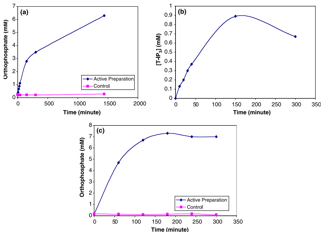
Figure 2. Dephosphorylation kinetic studies. (a) Progress curve showing release of ortho-P during the 3-phytase catalyzed dephosphorylation of T-IP 5 (2). (b) Progress curve showing accumulation of T-IP 3 subsequent to its disappearance. The concentration of T-IP 3 was determined by using T-IP 5 (2) as the standard. (c) Progress curve showing ortho-P release for 3-phytase catalyzed dephosphorylation of myo -IP 6 (1) (initial concentration 1.2 mM)—included for comparative purposes.
